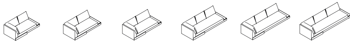
SENUBTRI202X 202 x 96 H79 79.53" x 37.80" H31.10" IZQ. SENUBTRI217X 217 x 96 H79 85.43" x 37.80" H31.10" IZQ. SENUBTRI227X 227 x 96 H79 89.37" x 37.80" H31.10" IZQ. SENUBTRI278X 278 x 96 H79 109.45" x 37.80" H31.10" IZQ. SENUBTRI308X 308 x 96 H79 121.26" x 37.80" H31.10" IZQ. SENUBTRI328X 328 x 96 H79 129.13" x 37.80" H31.10" IZQ. Left corner, right tray. Angle gauche, plateau droit. Rincón izquierdo, bandeja derecha.
