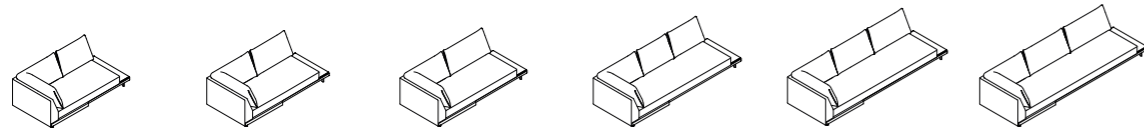
SENURI202X 202 x 96 H79 79.53" x 37.80" H31.10" IZQ. SENURI217X 217 x 96 H79 85.43" x 37.80" H31.10" IZQ. SENURI227X 227 x 96 H79 89.37" x 37.80" H31.10" IZQ. SENURI278X 278 x 96 H79 109.45" x 37.80" H31.10" IZQ. SENURI308X 308 x 96 H79 121.26" x 37.80" H31.10" IZQ. SENURI328X 328 x 96 H79 129.13" x 37.80" H31.10" IZQ. Left corner, right tray. Angle gauche, plateau droit. Rincón izquierdo, bandeja derecha.
